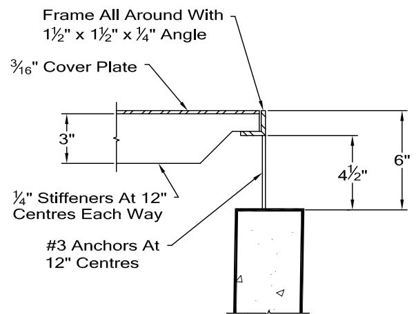
Cover Plate Support Detail
