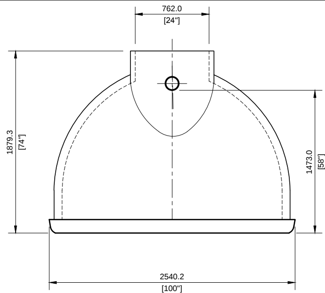
INLET END VIEW
