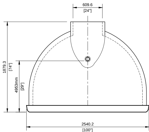
OUTLET END VIEW
