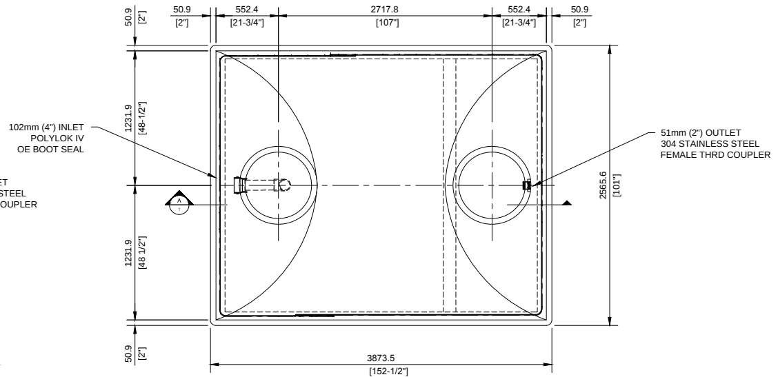
PLAN VIEW
