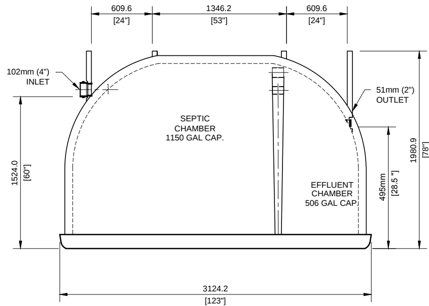
X-SECTION 1:30
