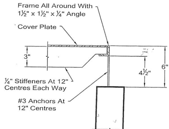
Cover Plate Support Detail
