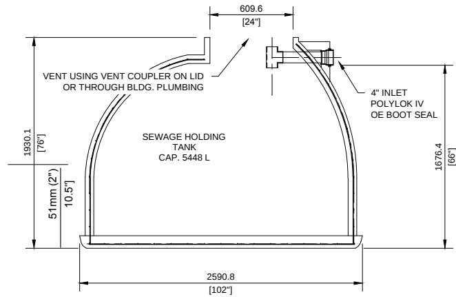
X-SECTION 1:30
