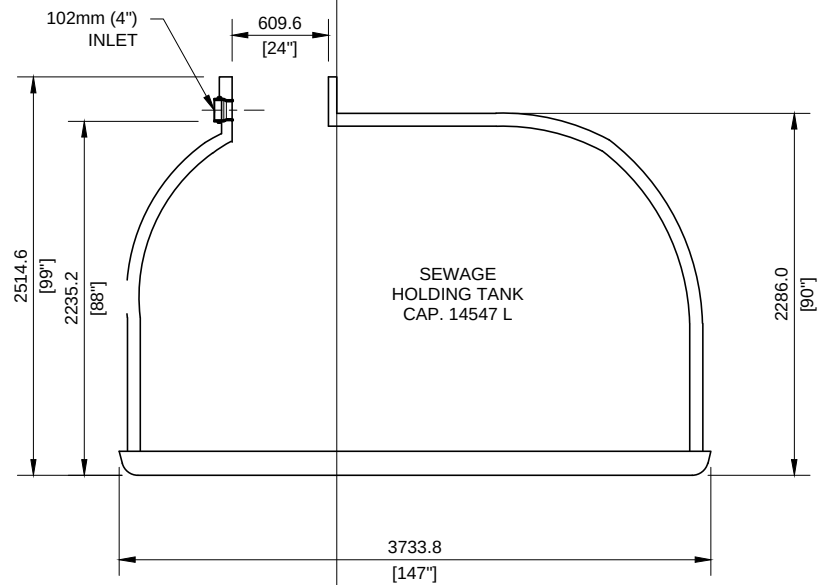
X-SECTION A 1:30
