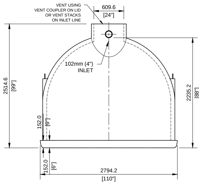
LEFT END VIEW
