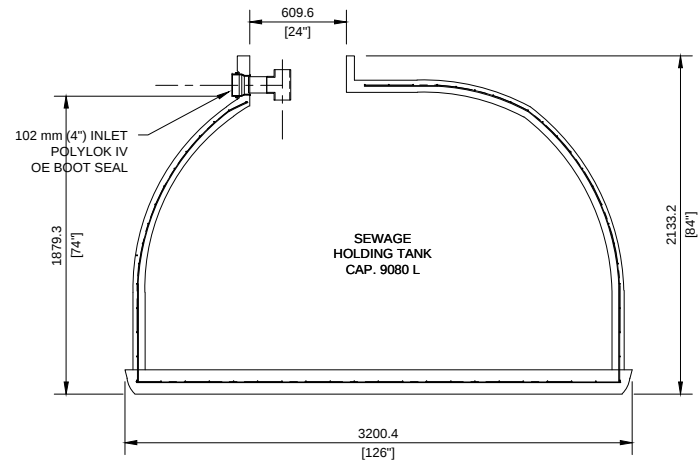
X-SECTION
